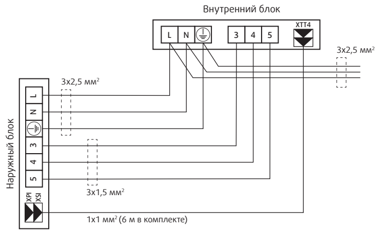
SYSPLIT FLOOR 24 HP Q
